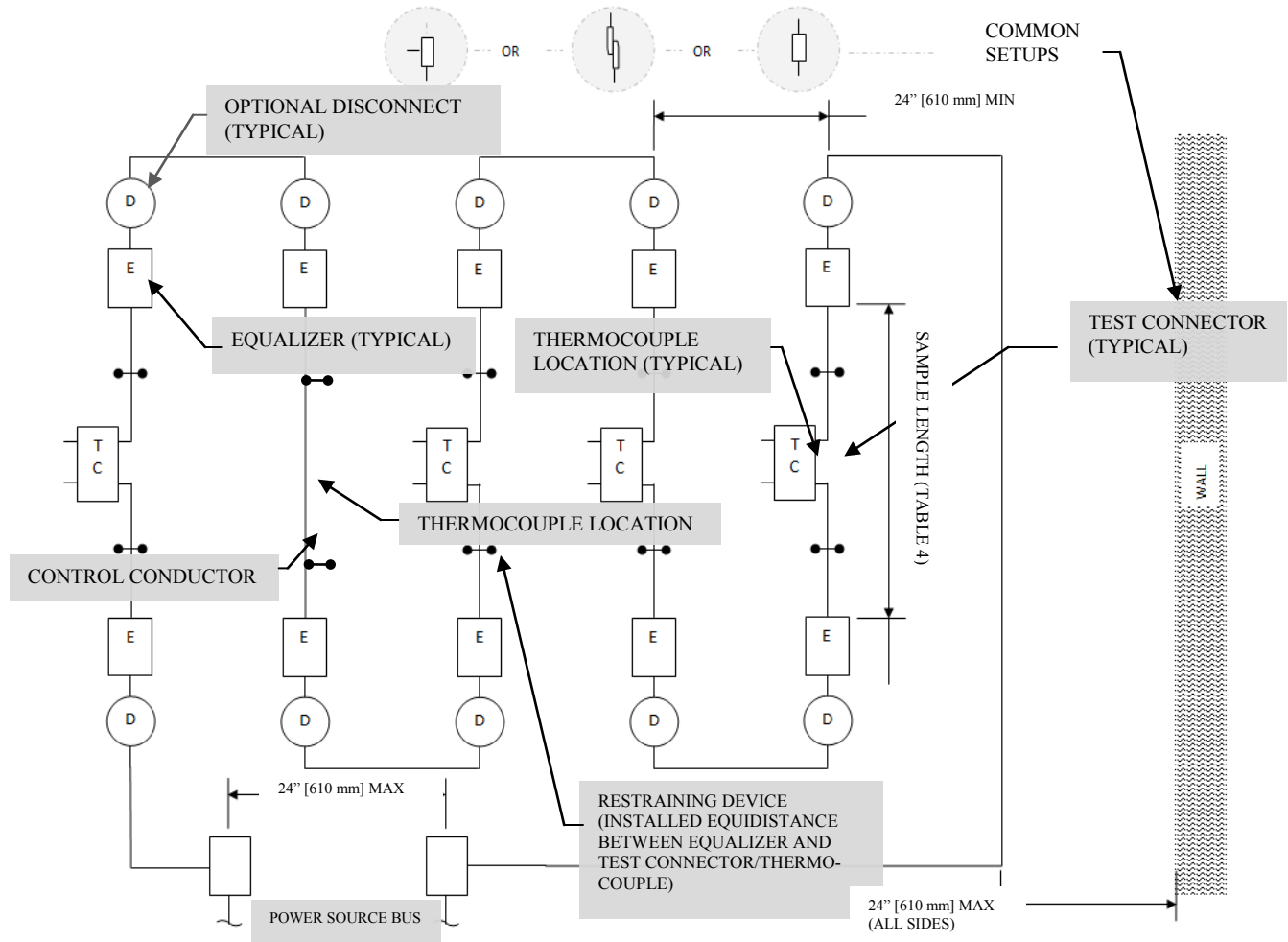
Figure 6—Typical sequential test loop
